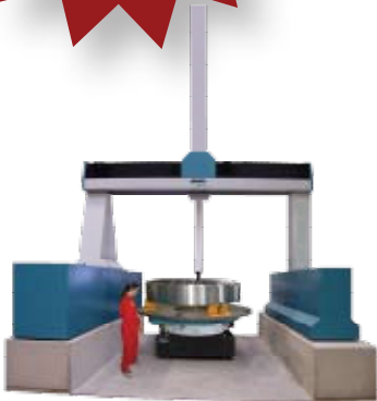
Wenzel LHF GMM (Gear Measuring Machine) Ø120" x 240" length x 80" height
